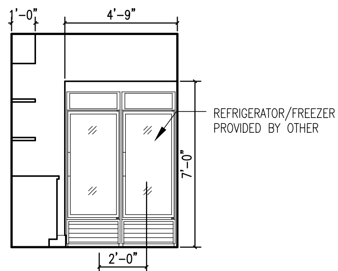
7 LG SUNDRY/ MARKETPLACE PLAN VIEW 1/4"=1'-0"
