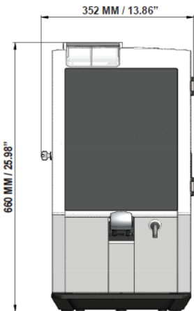
Esprecious 12 (shown open): Grinder (1), Whole bean hopper (1); holds up to 3.0 lbs., Soluble canisters (2); holds up to 2.0 lbs. each. Esprecious 22: Grinder (2), Whole bean hopper (2); holds up to 1.5 lbs. each. Soluble canisters (2); holds up to 2.0 lbs. each.
