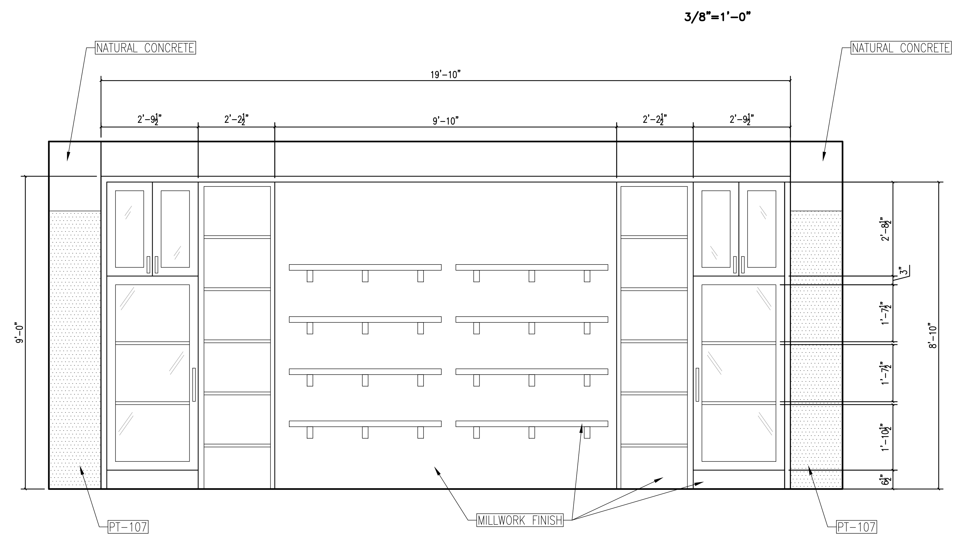
5 MARKETPLACE – NORTH WALL 3/8"=1'-0"
