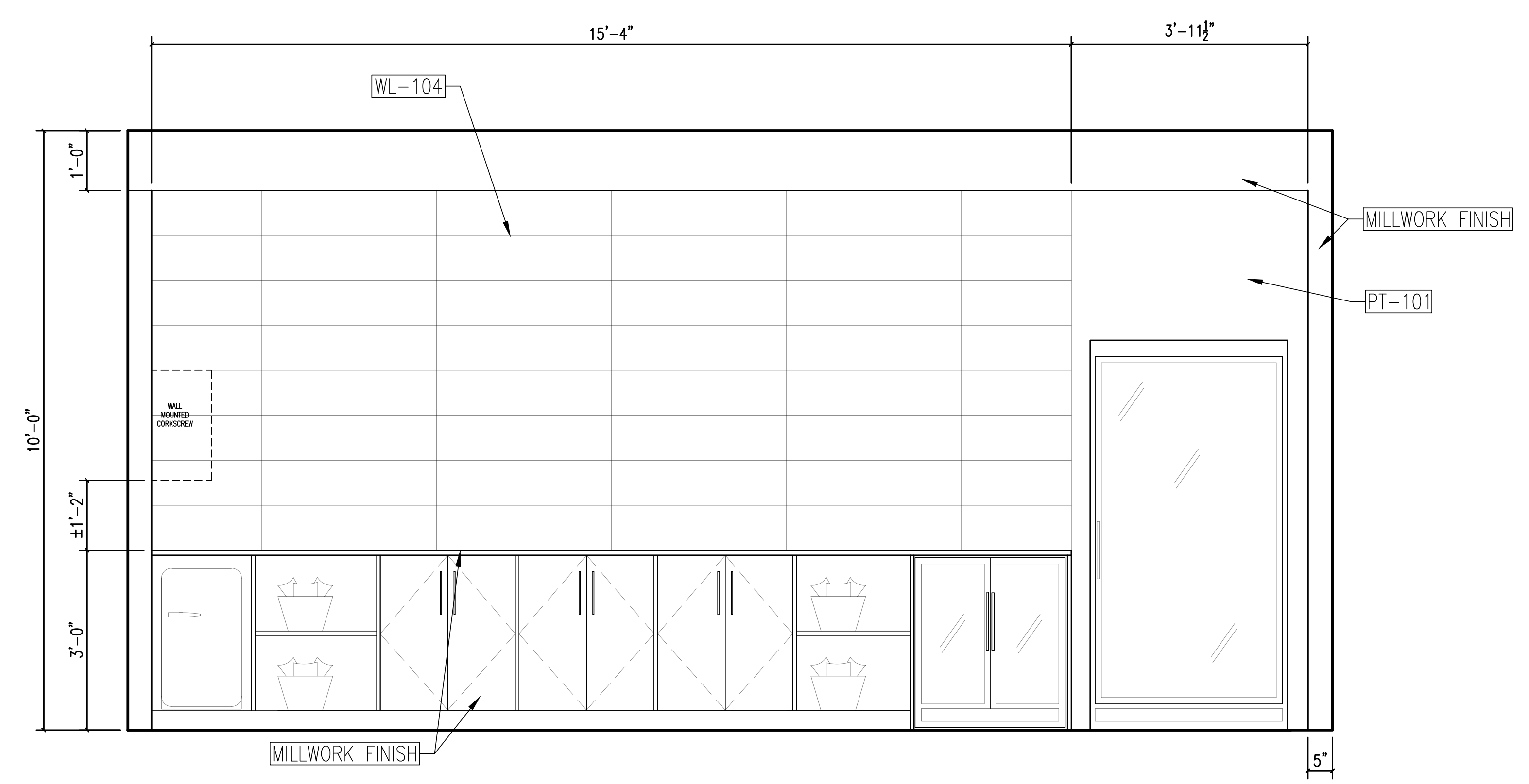
4 MARKETPLACE – SOUTH WALL 3/8"=1'-0"
