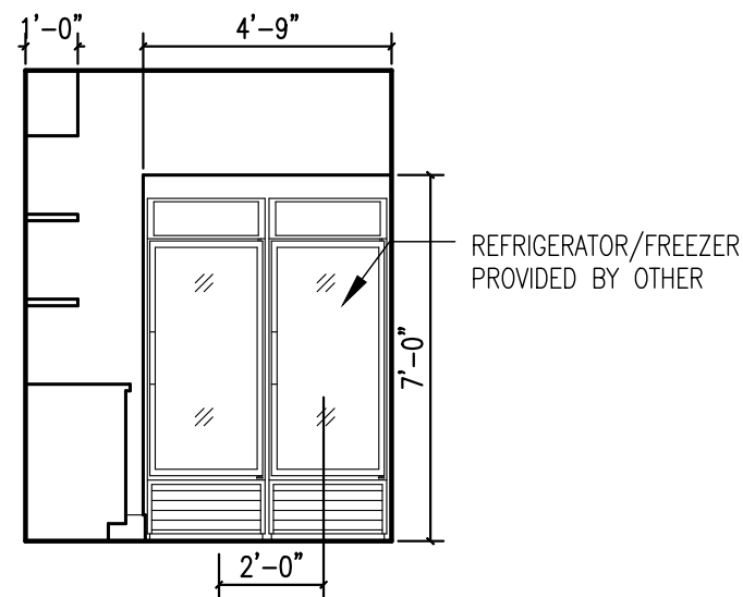
9 LG SUNDRY/MKTPLACE ELEVATION -COOLERS 1/4"=1'-0"
