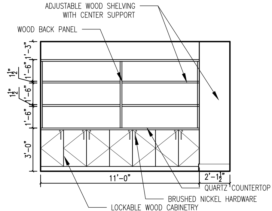
8 LG SUNDRY/MKTPLACE ELEVATION -SHELVING 1/4"=1'-0"
