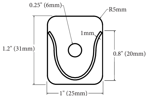
Mounting Bracket Front
