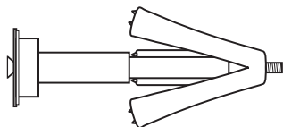
WINGITS® MASTER Anchor (MAW35FH) (2)
