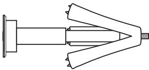
WINGITS® MASTER Anchor (MAW40FH) (3)
