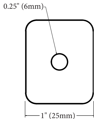
Mounting Bracket Back
